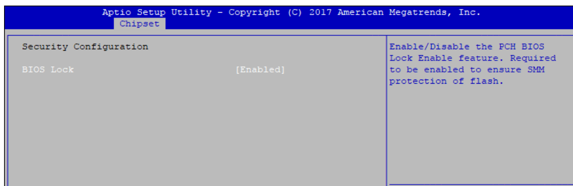
Figure 4-4-2-3 : Security Settings
