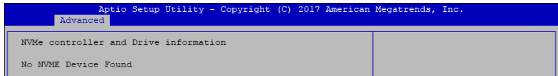
Figure 4-3-15 : NVMe Settings
