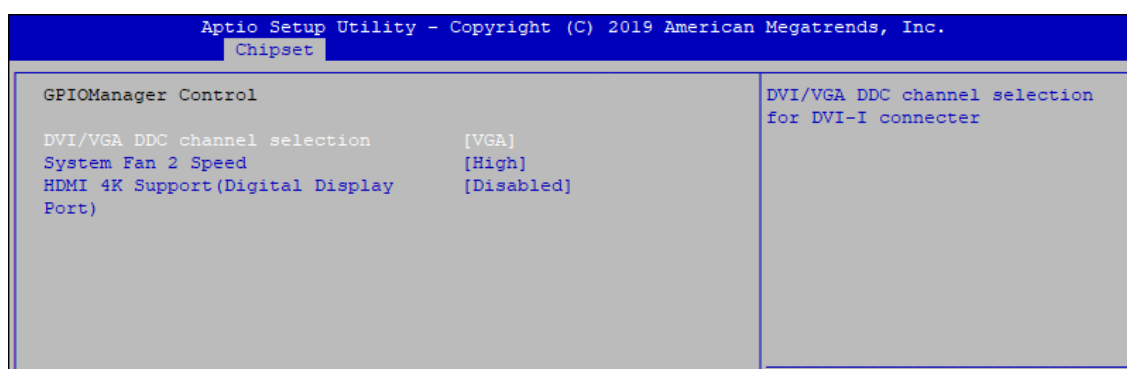
Figure 4-4-3 : GPIOManager Configuration
