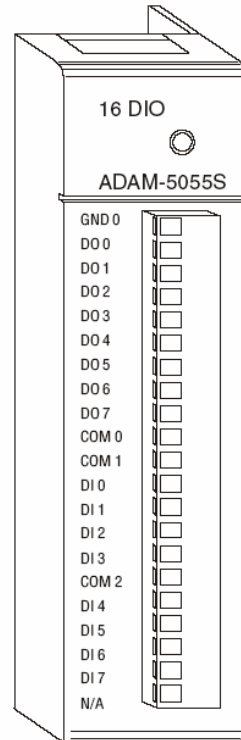
Figure 4.15 ADAM-5055S Module Front View
