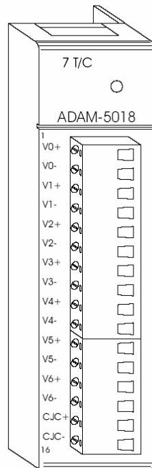
Figure 1.21 ADAM-5018 Module Front View
