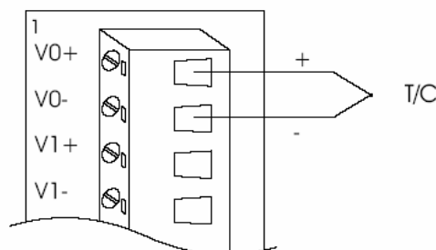
Figure 1.22 Thermocouple Input
