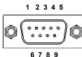
Figure 2.3 COM Connector
