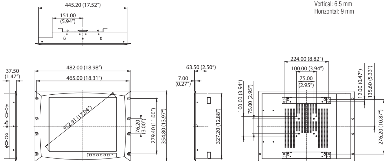
Panel Cut-out Dimensions: FPM-3171G: 447.5 x 329.5 mm (17.62" x 12.97")
