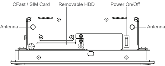
Front I/O
