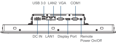
Rear I/O
