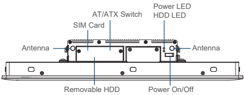
Front I/O
