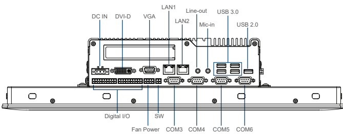
Front I/O
