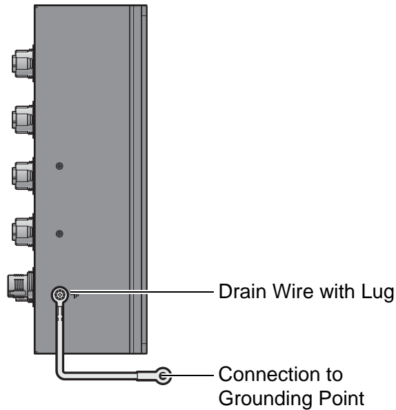
Figure 2.4 Grounding Connection, Chassis Left Side View
