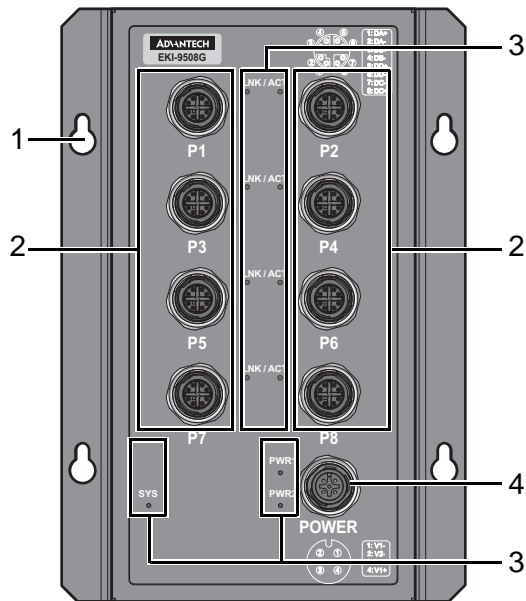
Figure 1.5 Front View
