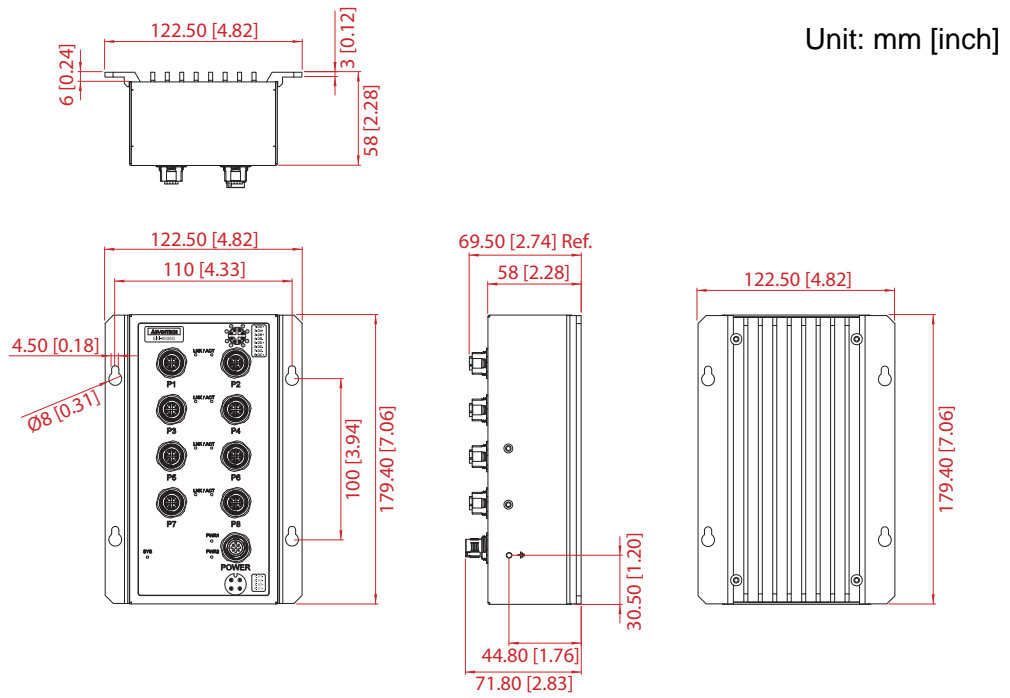
Figure 1.14 EKI-9508G-H/EKI-9508G-L Dimensions
