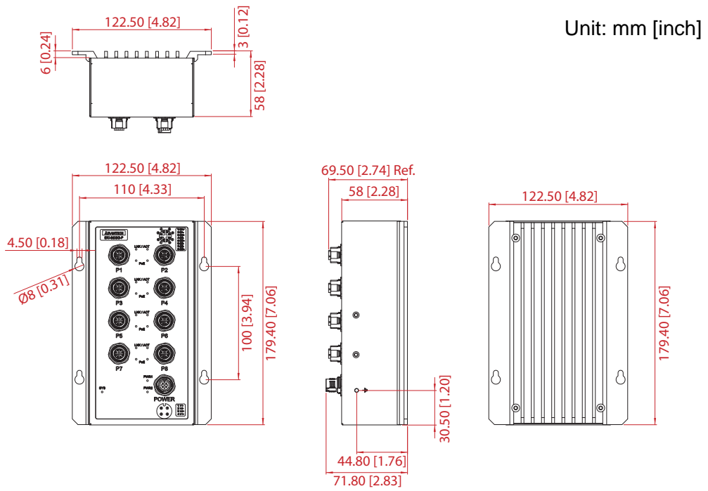
Figure 1.17 EKI-9508G-PH/EKI-9508G-PL Dimensions
