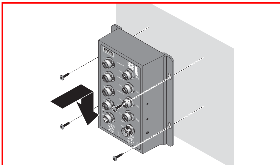
Figure 2.2 Switch Installation
