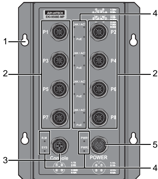
Figure 1.3 Front View
