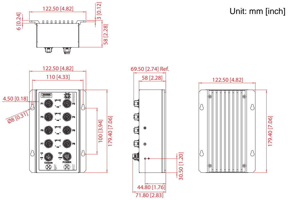
Figure 1.16 EKI-9508G-MPH/EKI-9508G-MPL Dimensions
