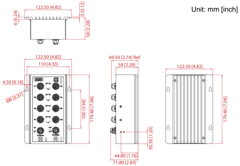
Figure 1.12 EKI-9508E-MPH/EKI-9508E-MPL Dimensions
