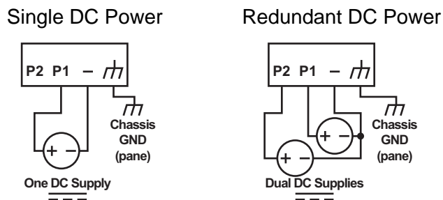
Figure 2.3 Power Wiring for EKI-9508 Series
