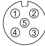
Figure 2.9 M12 A-Coded Connector Pin Assignment
