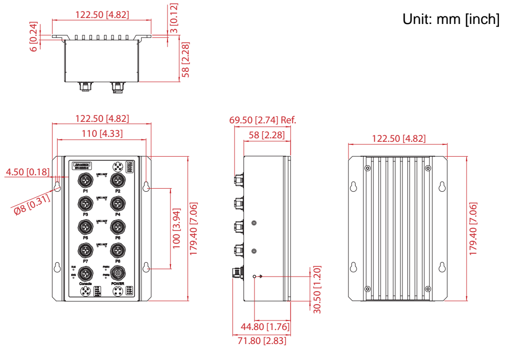
Figure 1.11 EKI-9508E-MH/EKI-9508E-ML Dimensions
