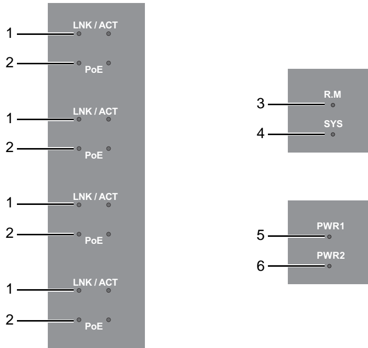
Figure 1.9 System LED Panel
