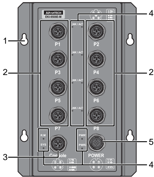
Figure 1.2 Front View
