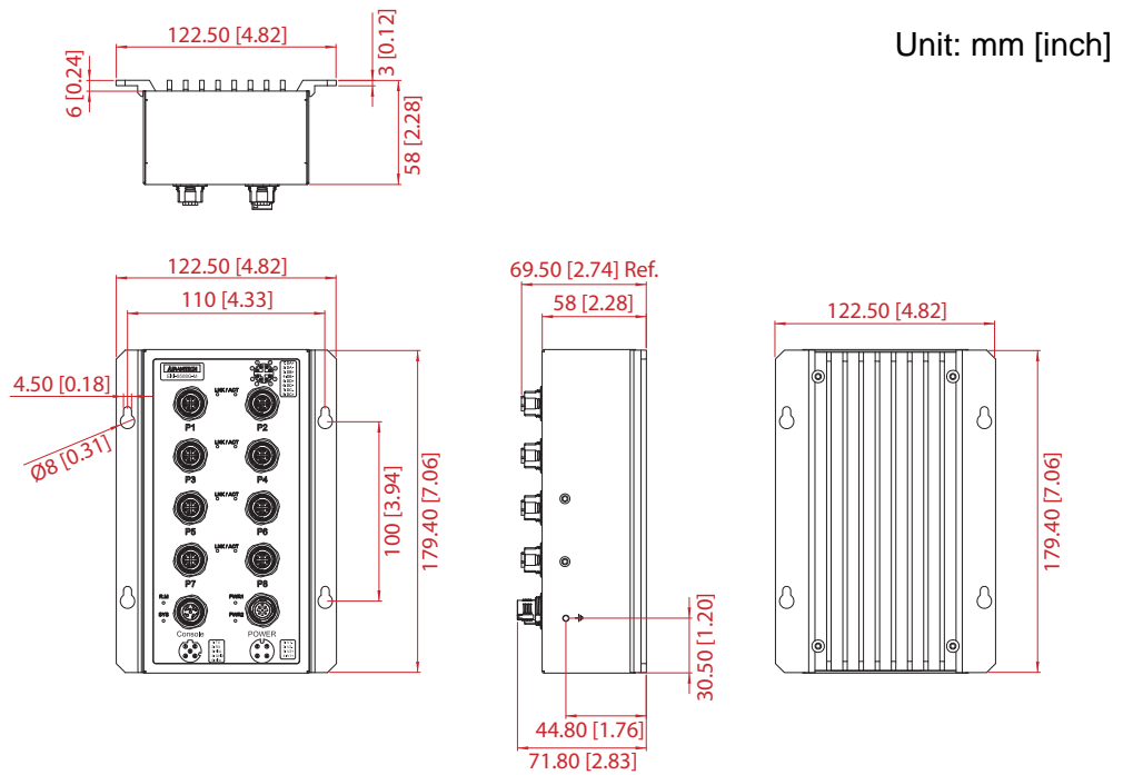
Figure 1.15 EKI-9508G-MH/EKI-9508G-ML Dimensions
