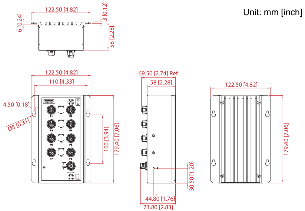
Figure 1.13 EKI-9508E-PH/EKI-9508E-PL Dimensions
