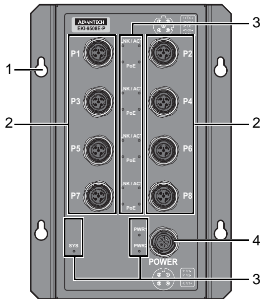
Figure 1.4 Front View
