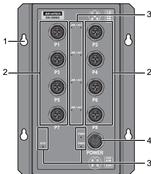
Figure 1.1 Front View
