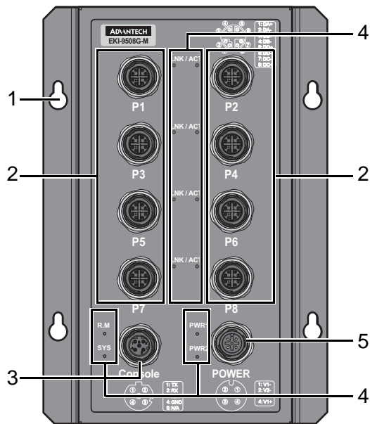
Figure 1.6 Front View
