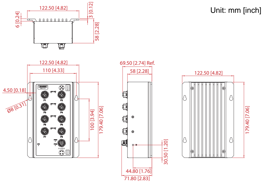
Figure 1.10 EKI-9508E-H/EKI-9508E-L Dimensions
