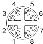
Figure 2.8 M12 X-Coded Connector Pin Assignment
