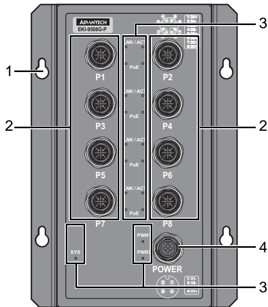
Figure 1.8 Front View
