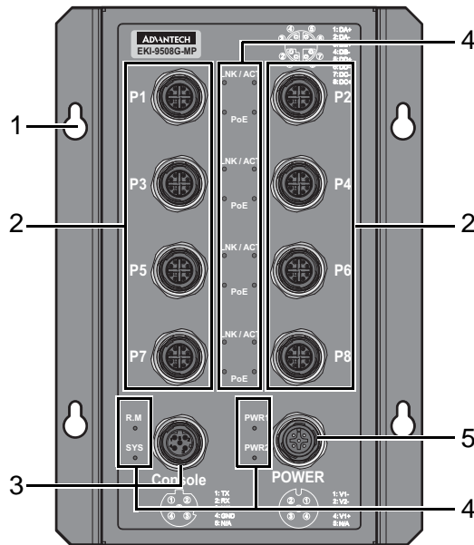
Figure 1.7 Front View
