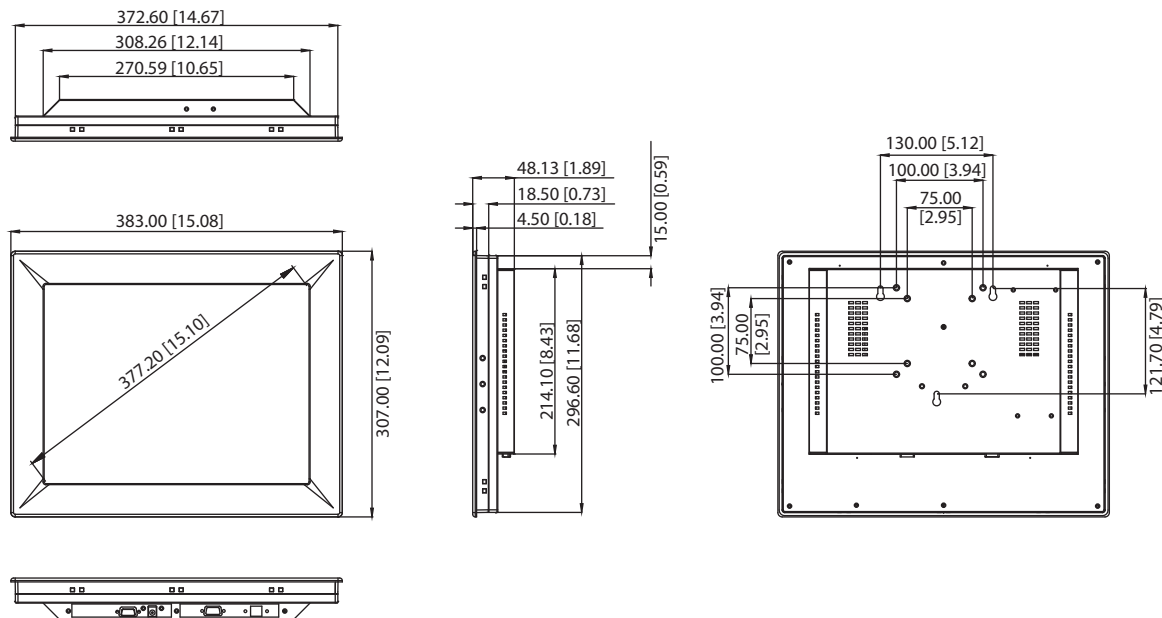
Panel Cut-out Dimensions: 374.6 x 298.6 mm (14.75" x 11.75")
