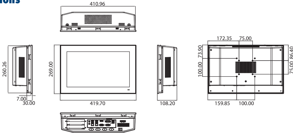
Panel Cutout Dimensions: 413 x 262 mm (16.25 x 10.31 in)
