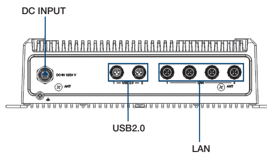
Rear Panel
