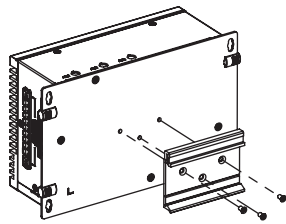
DIN-Rail Assembly
