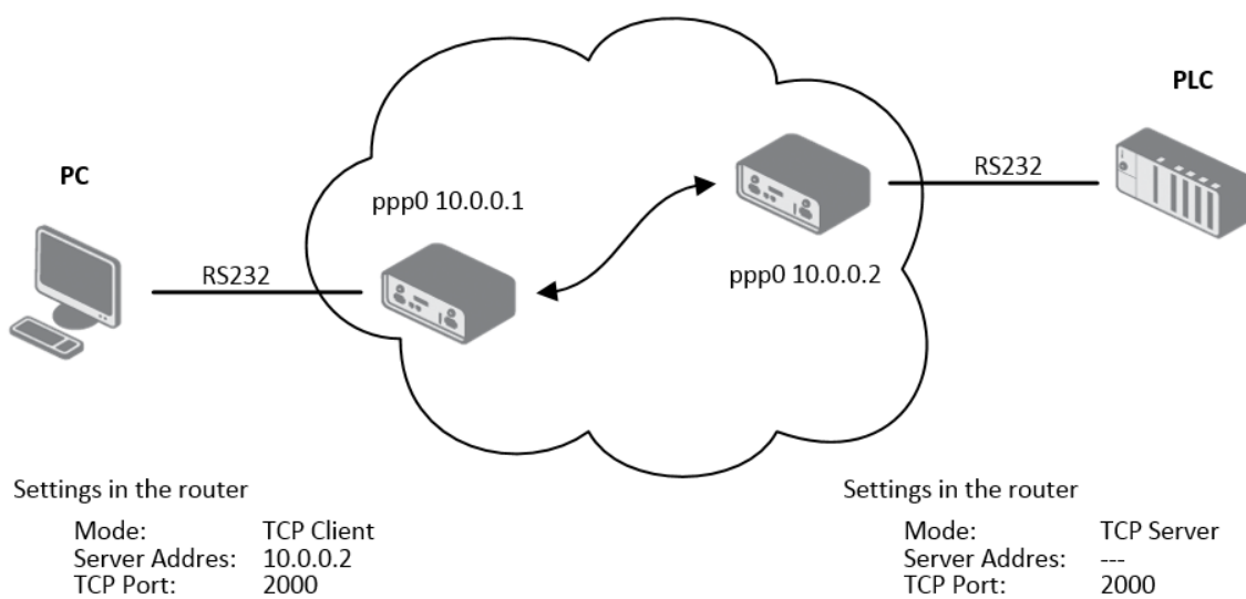
Figure 64: Example of serial port extension
